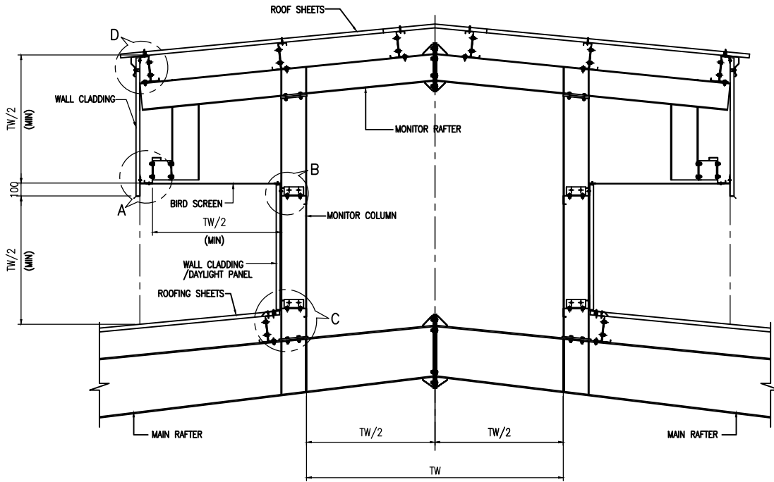
ROOF MONITOR (TYPE-C) FLUSH GIRT
