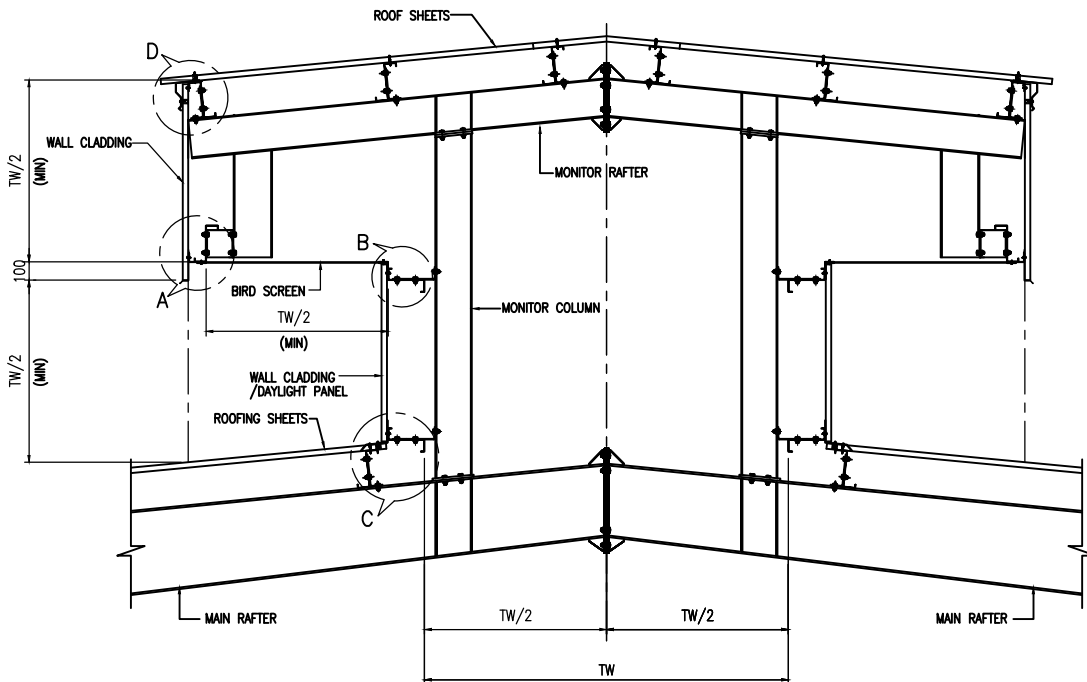
ROOF MONITOR (TYPE-D) BY-FRAME GIRT
